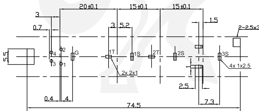
Recommended P.C.B. Layout Bottom view
