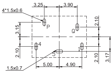
Recommended P.C.B. layout top view, tolerances: ±0.05
