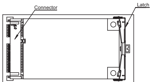
Mounting on board condition
