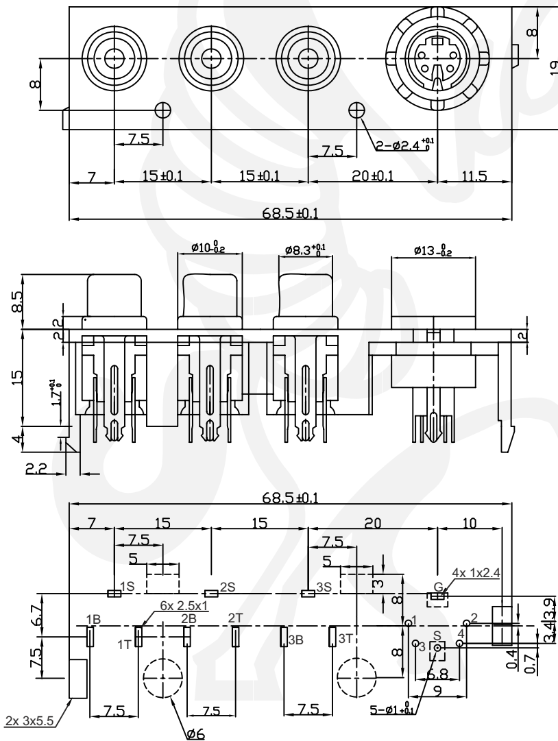
Recommended P.C.B. Layout Bottom view
