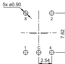
Recommended P.C.B. layout (3+2)
