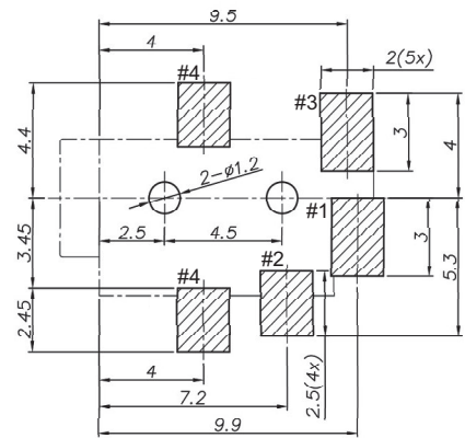
Recommended P.C.B. layout bottom view, tolerances: ±0.05
