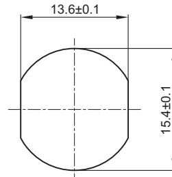
Recommended panel cut-out PG9 thickness 4.0 max.
