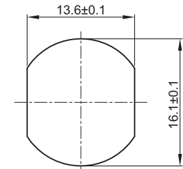
Recommended panel cut-out M16 thickness 4.0 max.
