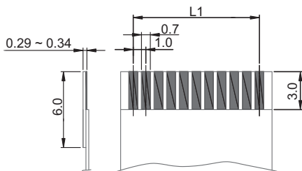
Accommodated FFC/FPC
